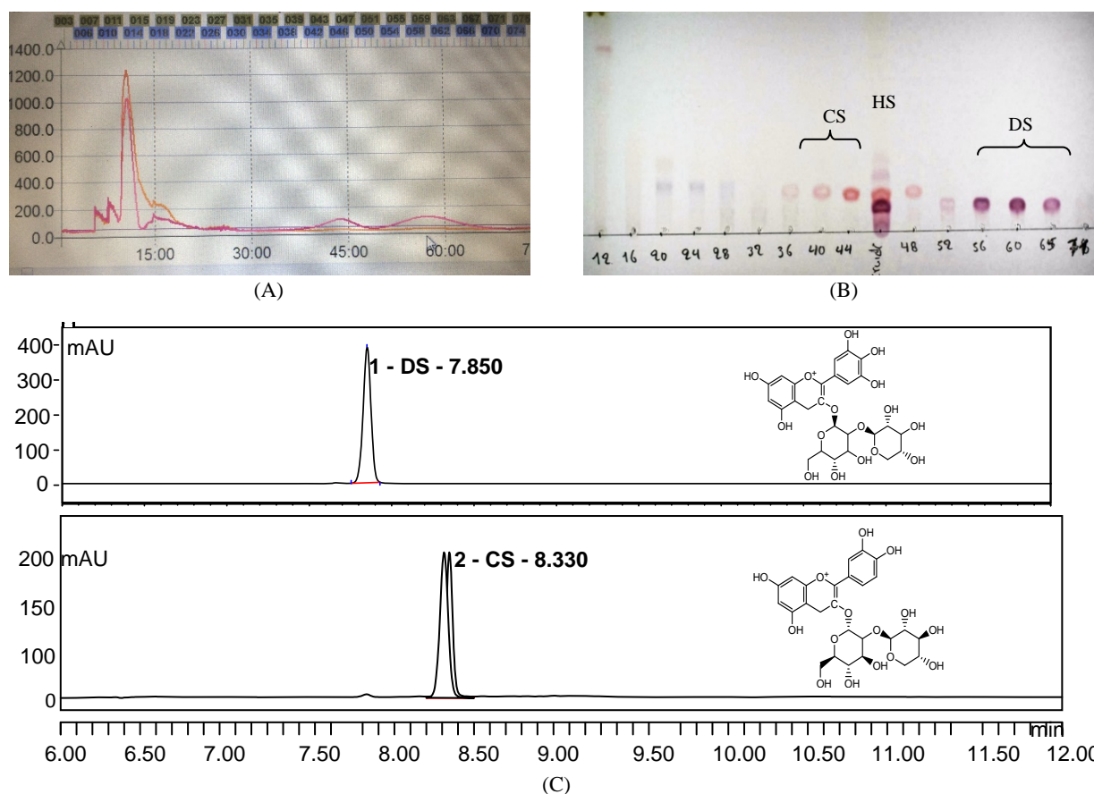
Fig. 1 CPC chromatogram of (A) Standard elution separation corresponding (B) Thin layer chromatography (TLC) fractograms and corresponding (C) UHPLC (Ultra high performance liquid chromatography) spectrum at 520 nm for DS and CS fraction.
