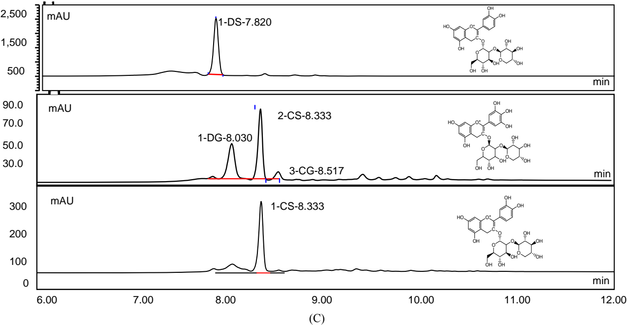
Fig. 2 CPC chromatogram of (A) pHZR corresponding (B) Thin layer chromatography (TLC) fractograms and corresponding (C) UHPLC spectrum at 520 nm for DS and CS fraction.
