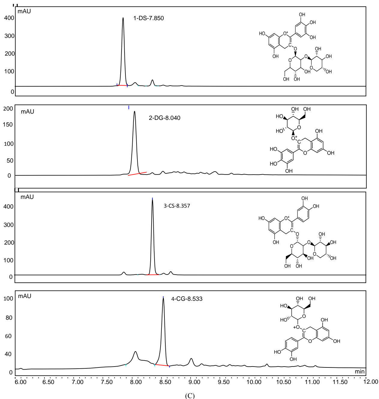
Fig. 3 CPC chromatogram of (A) Strong ion chromatography (SIX CPC) corresponding (B) Thin layer chromatography (TLC) fractograms and corresponding (C) UHPLC spectrum at 520 nm for DS, DG, CS ,CG fraction.
