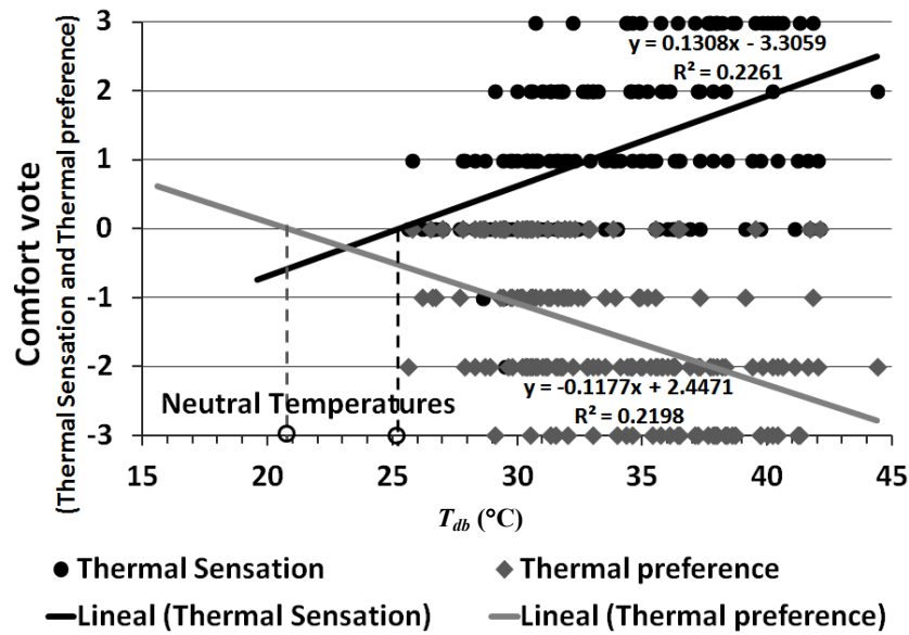
Fig. 7 Determination of T_n and CR by adaptive conventional method (example: Mexicali/May-October 2006).
