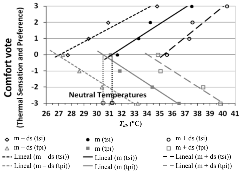
Fig. 8 Determination of T_n and CR by ATSI method (example: Mexicali/May-October 2006).
