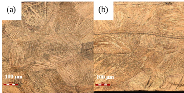
Fig. 4 Confocal micrograph of the Cu-14Al-4Ni alloy, without DCT, with (a) 100 cycles and (b) 500 cycles.
