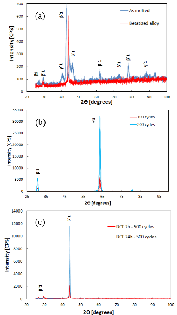
Fig. 1 Results of the XRD analyses of: (a) as melted and betatized samples; (b) samples without DCT after 100 and 500 cycles; (c) samples with DCT time of 2h and 24 h after 500 cycles.
