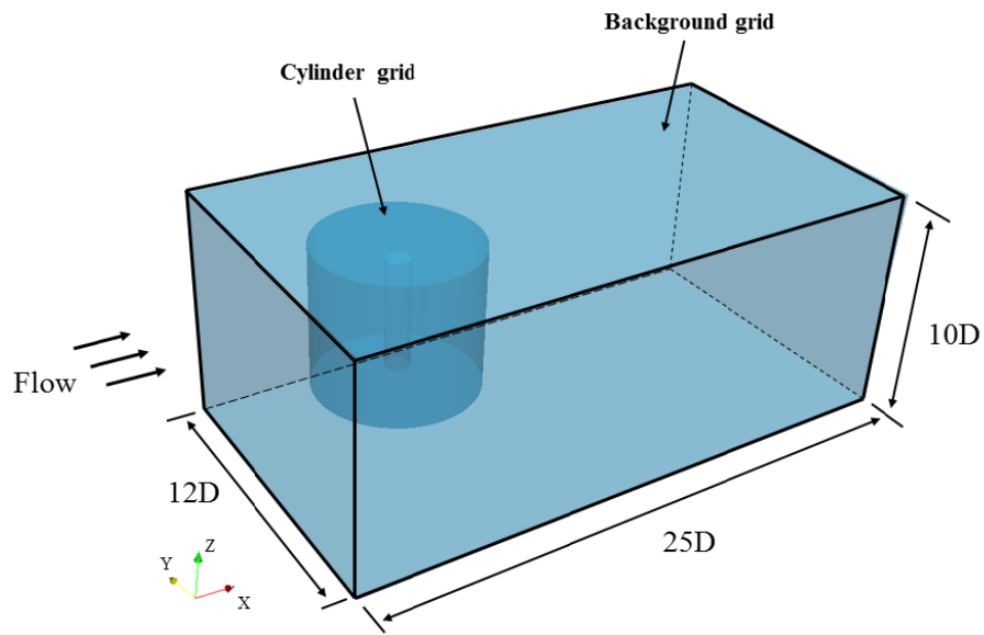
Fig. 2 Computational domain.
