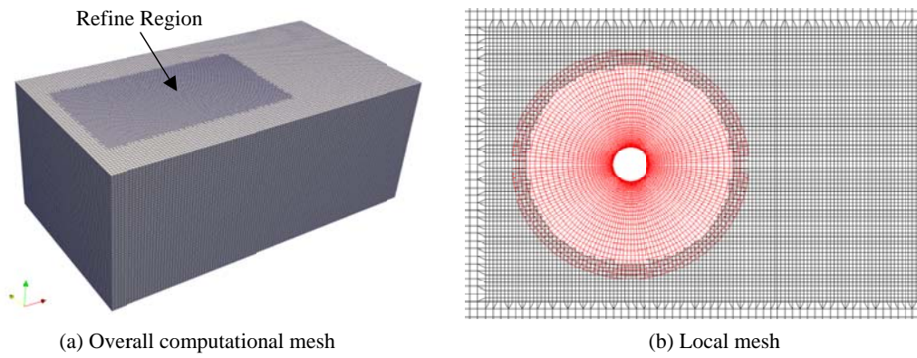
Fig. 3 Computational mesh.
