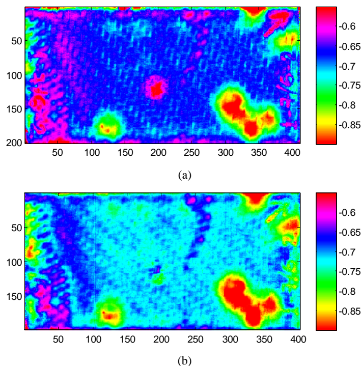
Fig. 3 PPT phase thermograms obtained from Testpiece 2 (code 1-7/6-2) in reflection mode: (a) As-impacted at -70 °C; (b) As-repaired at 55 °C under direct infrared light.
