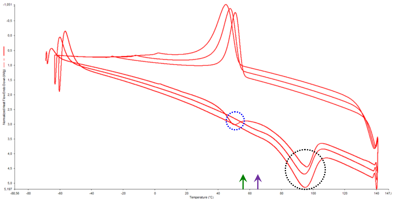
Fig. 5 DSC curves for a 0.5 mm-thick E-MAA film ballistically impacted at ambient temperature and autonomously recovered. Order-disorder transition temperature and melting temperature range of pre-damaged and immediately self-healed E-MAA film indicated by dashed blue and black circles, respectively. Minimum and maximum temperatures where thermally-activated healing was observed in hybrid laminate are indicated by green (55 °C) and purple (70 °C) arrows.
