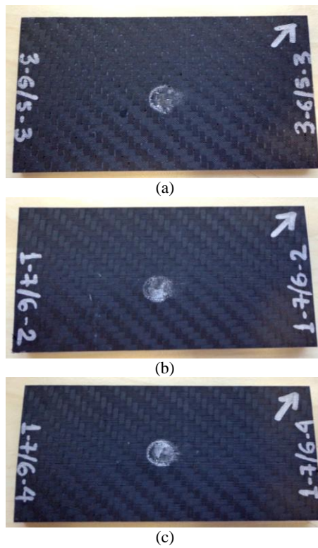
Fig. 1 Front (impacted) face of test coupons after ballistic impact at approximately -70\text{ }^{\circ}\text{C} : (a) Testpiece 1, coded 3-6/5-3; (b) Testpiece 2, coded 1-7/6-2; (c) Testpiece 3, coded 1-7/6-4.
