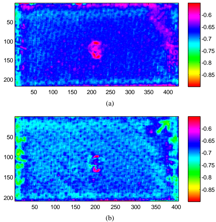
Fig. 2 PPT phase termograms obtained from Testpiece 1 (code 3-6/5-3) in reflection mode: (a) As-impacted at -70\text{ }^{\circ}\text{C} ; (b) As-repaired at 70\text{ }^{\circ}\text{C} in convective furnace.
