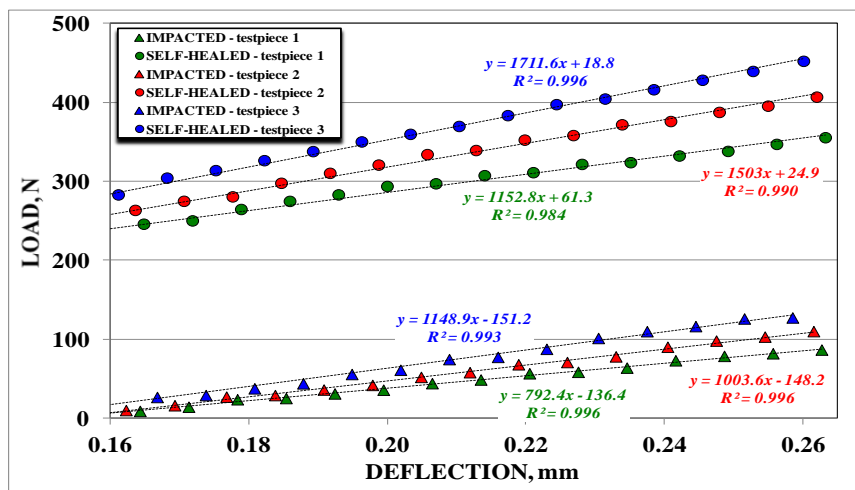
Fig. 6 Load-load line deflection graph from 4-point flexural testing of as-impacted hybrid laminate and after thermally-activated self-healing of interleaved ionomeric thermoplastic E-MAA film.
