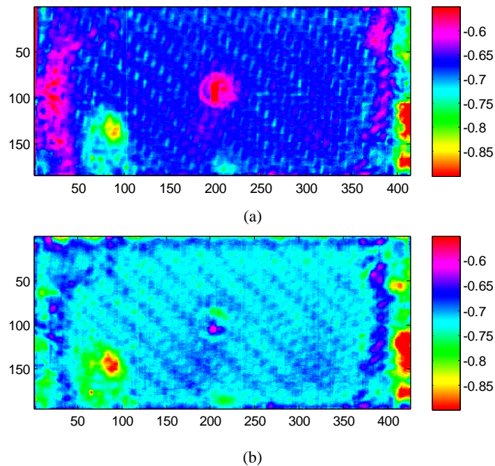
Fig. 4 PPT phase thermograms obtained from Testpiece 3 (code 1-7/6-4) in reflection mode: (a) As-impacted at -70 °C; (b) As-repaired at 70 °C under direct infrared light.
